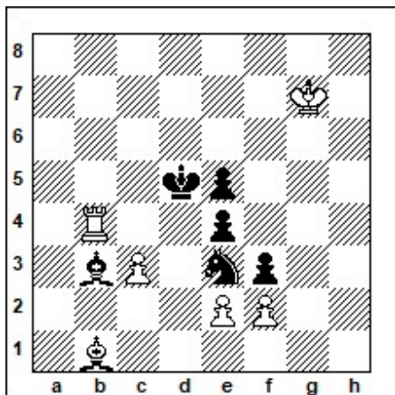
h#3, 2 solutions (6 + 6)
