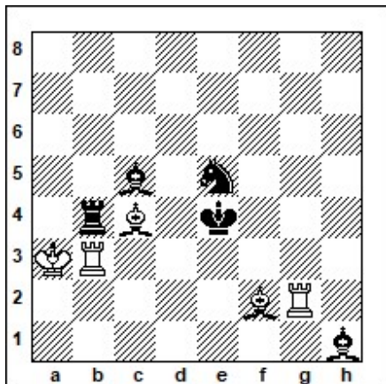
h#2, 2 solutions (5 + 5)
