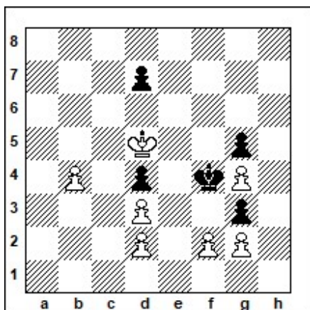
h#5 (7 + 5)
